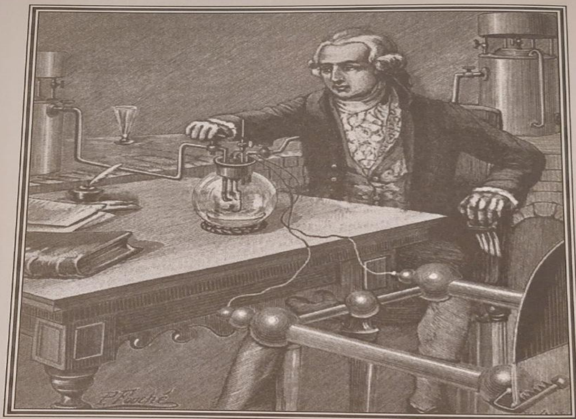
Lavoisier's water formation experiment 335
